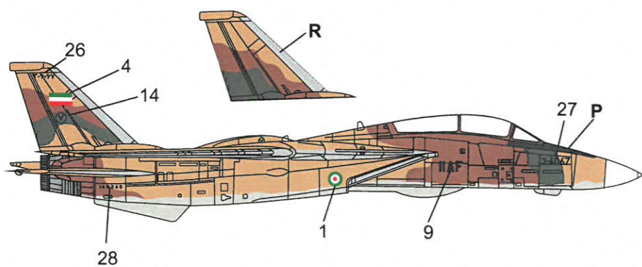
F-14A 160365/3-6067, 73 rd TFS, Imperial Iranian Air Force - IIAF; TBF 7 Shiraz, 1978, before the islamic revolution During the war with Iraq, this aircraft was credited with at least 11 aerial victories. The standard combat load consisted in 2 AIM-54A Phoenix, 3 AIM-7-E4 Sparrow and 2 AIM-9P Sidewinder AAMs.
