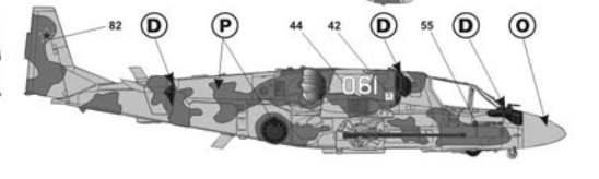
Place of technical stencil on serial Ka-50 helicopter
