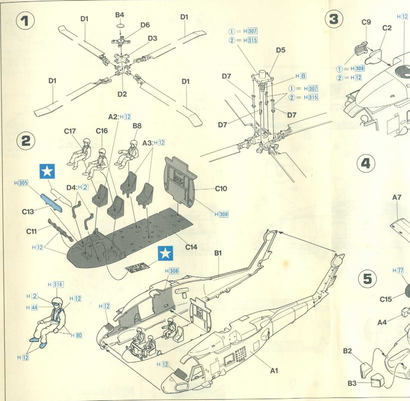
SH-60B SEAHAWK
