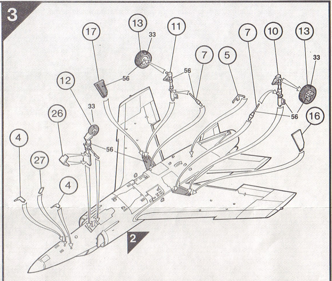
DASSAULT SUPER ETENDARD. 2 ESCUADRILLA DE CAZA Y ATAQUE, 3 ESCUADRA AERONAVAL. COMANDO AVIACION NAVAL ARGENTINA (ARGENTINE NAVAL AVIATION COMMAND), COMMANDANTE ESPORA AIR BASE, ARGENTINA, LATE 1982
