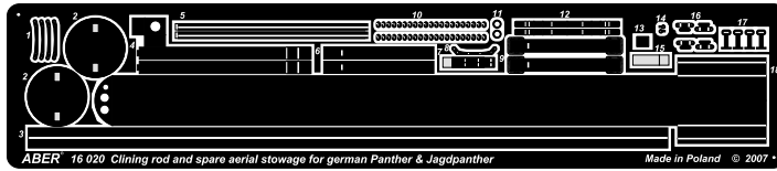
ABER 16 020 Cleaning rod and spare aerial stowage for german Panther & Jagdpanther
