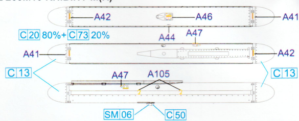
Wingtip P-72(R)
